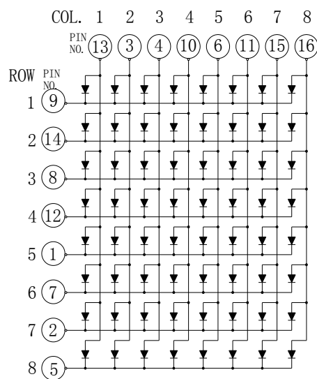
Common Row Cathode: KWM-R30881CAB
