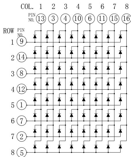
Common Row Anode: KWM-R30881AAB
