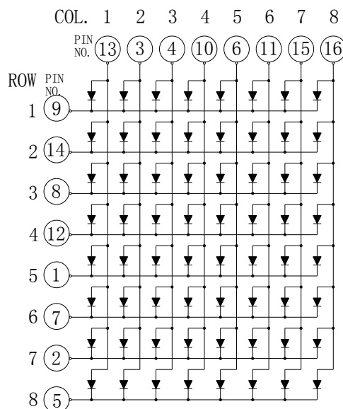
Common Row Cathode: KWM-50881CBB
