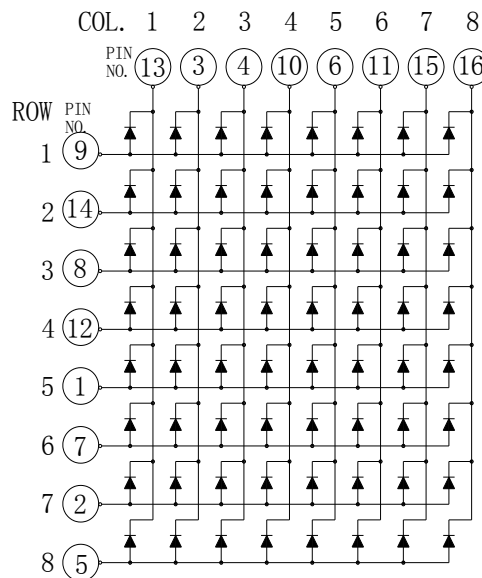
Common Row Cathode: KWM-50881CBB
