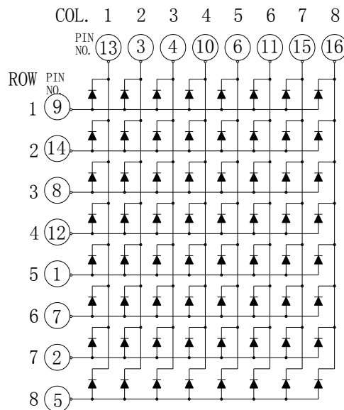
Common Row Cathode: KWM-50881CAB
