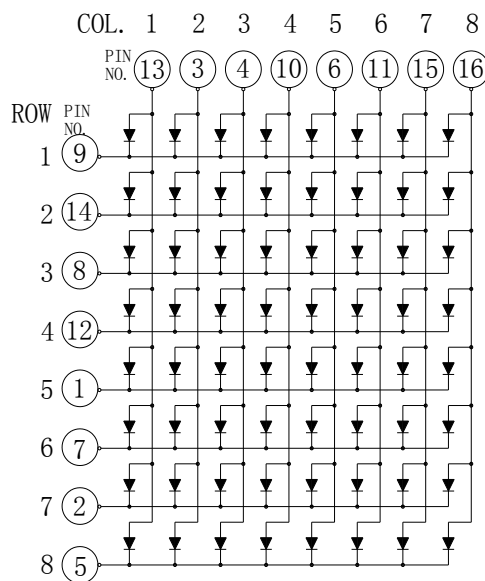
Common Row Cathode: KWM-50881CAB
