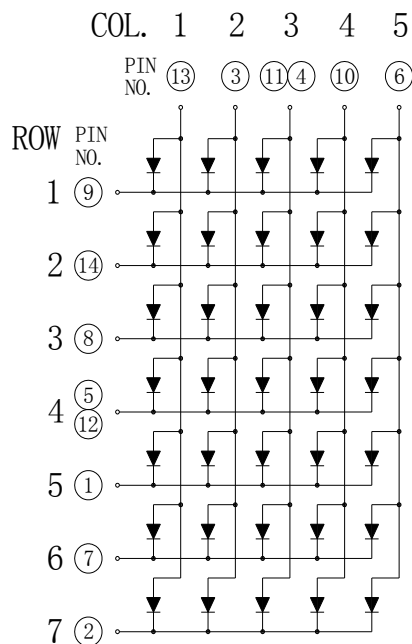
Common Row Cathode: KWM-30571CWB
