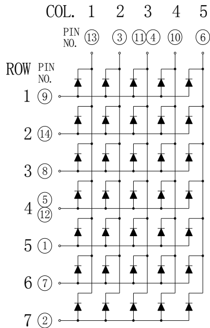
Common Row Anode: KWM-30571AVB
