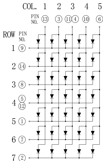
Common Row Cathode: KWM-30571CVB
