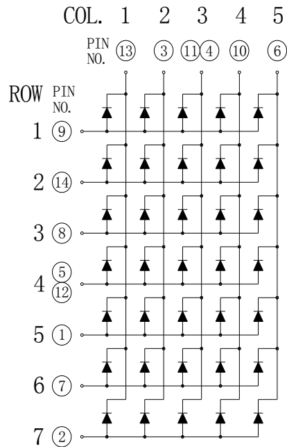
Common Row Anode: KWM-30571AAB
