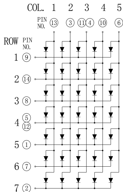
Common Row Cathode: KWM-30571CAB
