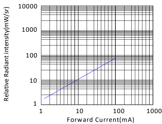
Fig. 3 - Relative Radiant Intensity vs. Forward Current
