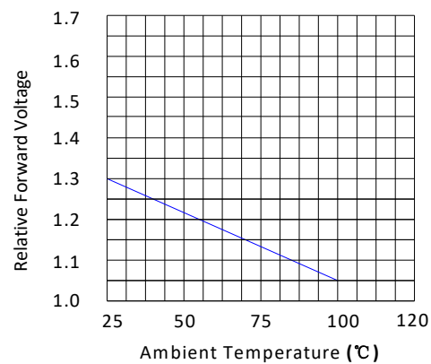
Fig. 4 - Forward Voltage vs. Ambient Temperature(°C)
