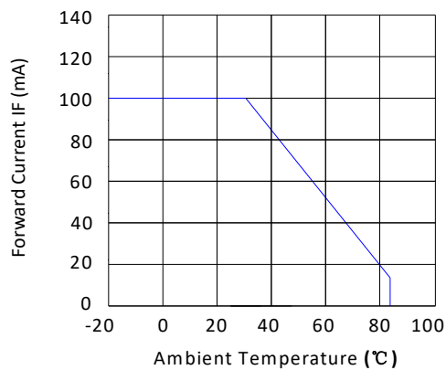
Fig. 5 - Forward Current vs. Ambient Temperature
