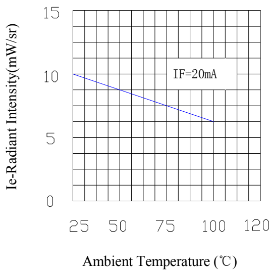
Relative Intensity & Ambient Temperature (°C)
